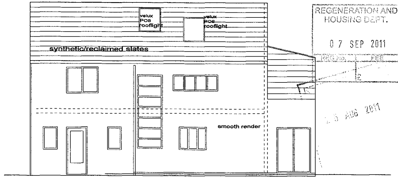
NORTH ELEVATION
