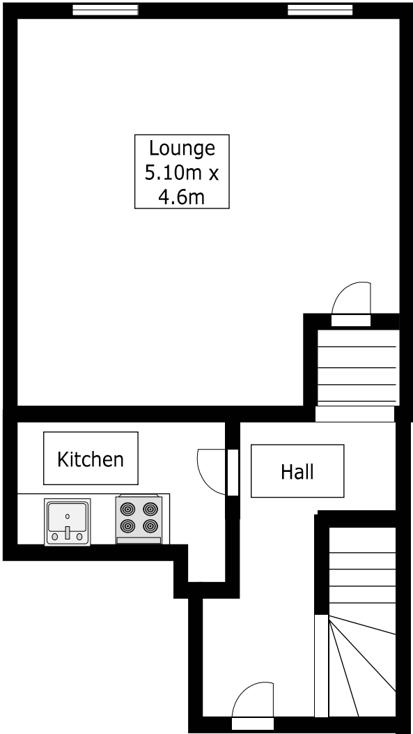
1st Floor
